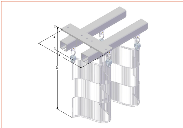
Sinus-shape curtain suspended on two rails side view
